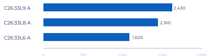
C26:33L Genset (1000 r/min) Max Cont Rating (kW)
